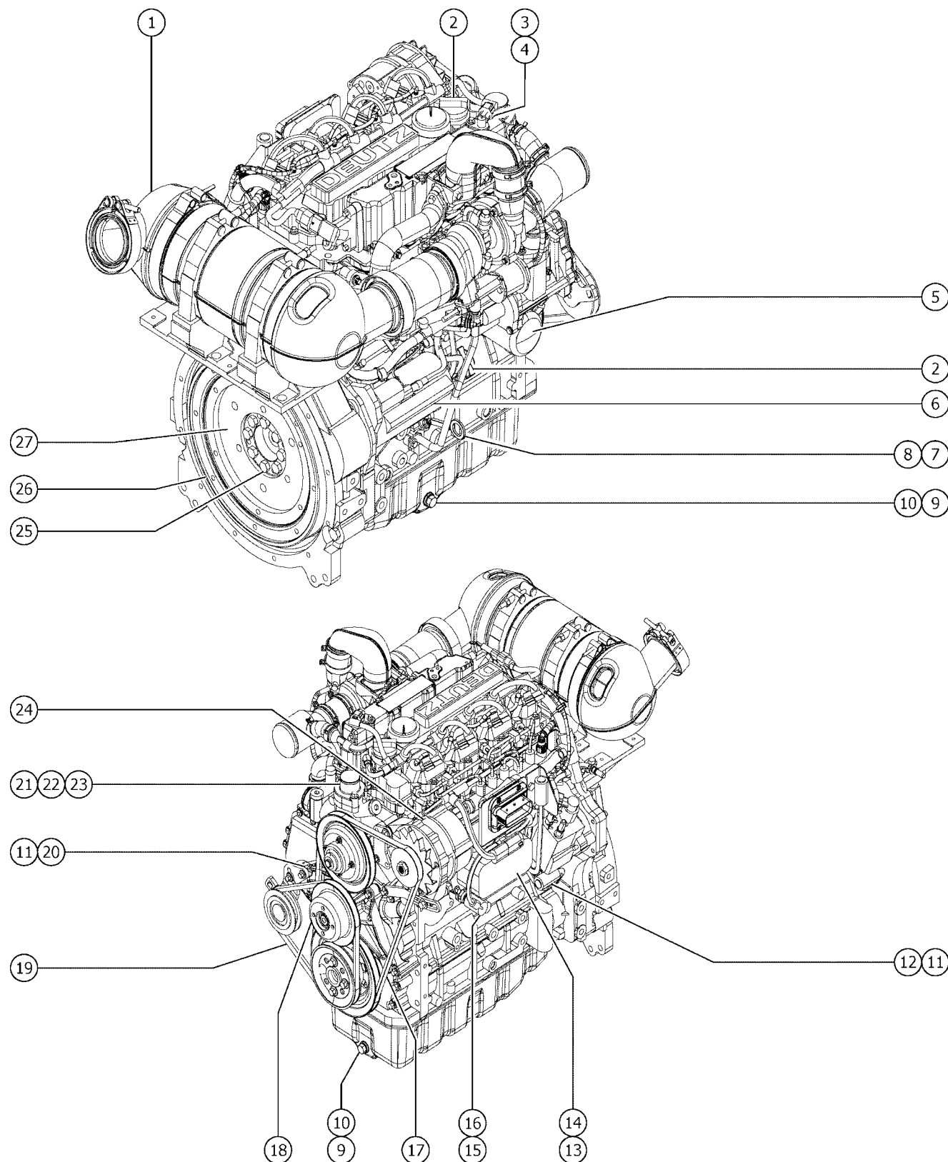
518.1 Deutz D2.9L4, View 1 (from SN S-65TX-101)
