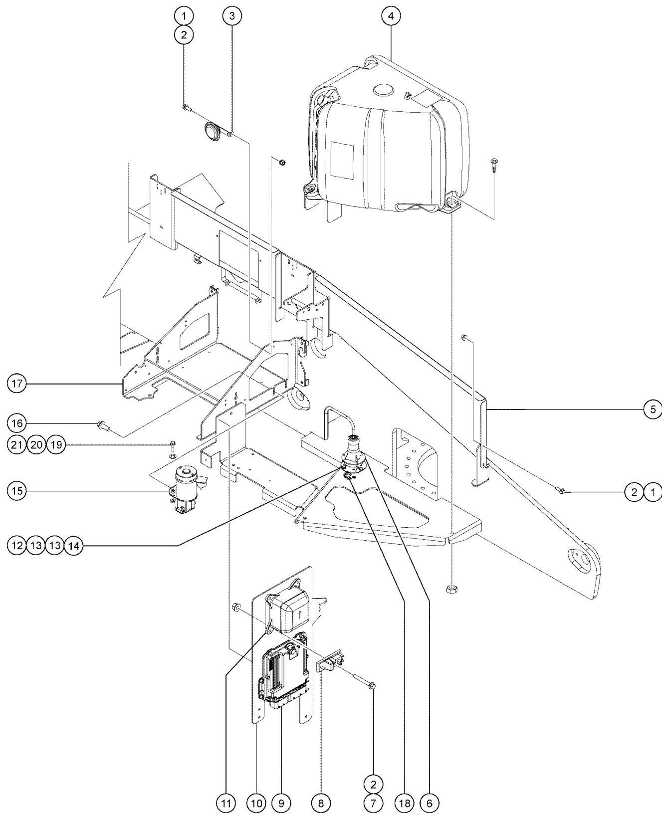
302.1 Tank Side - View 2
