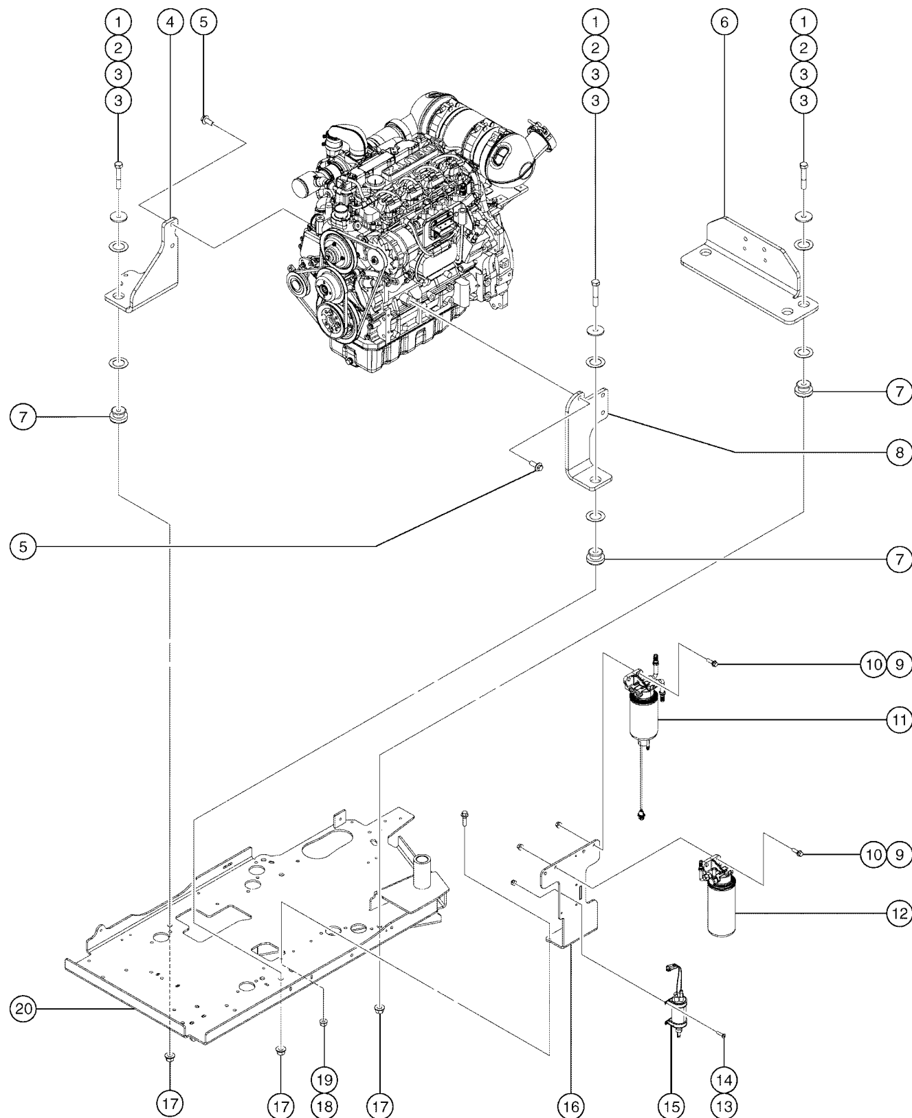
522.1 Deutz D2.9L4, View 5 (from SN S-65TX-101)
