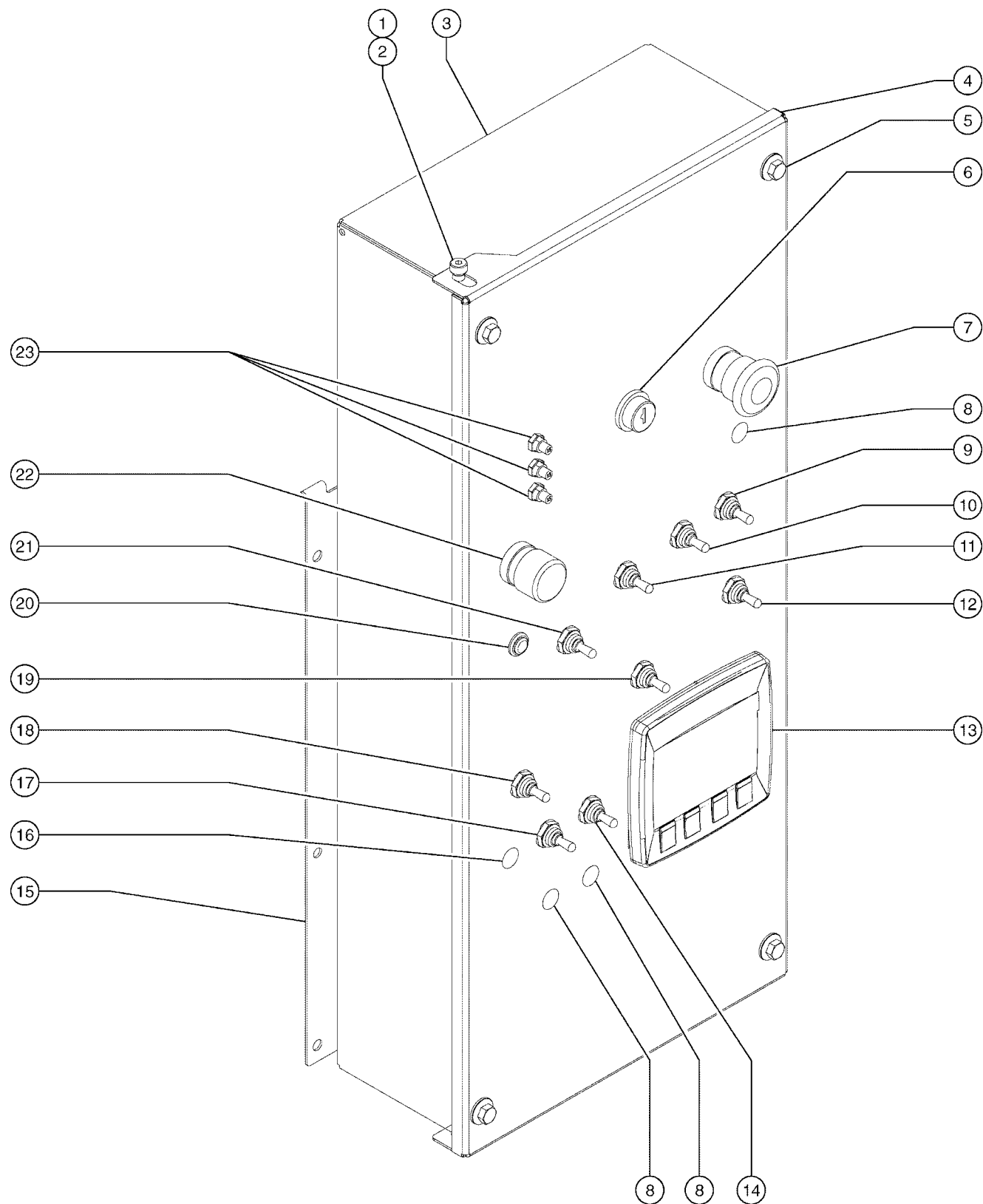
307.1 Ground Control Box, with LCD Readout Screen - View 1, External
