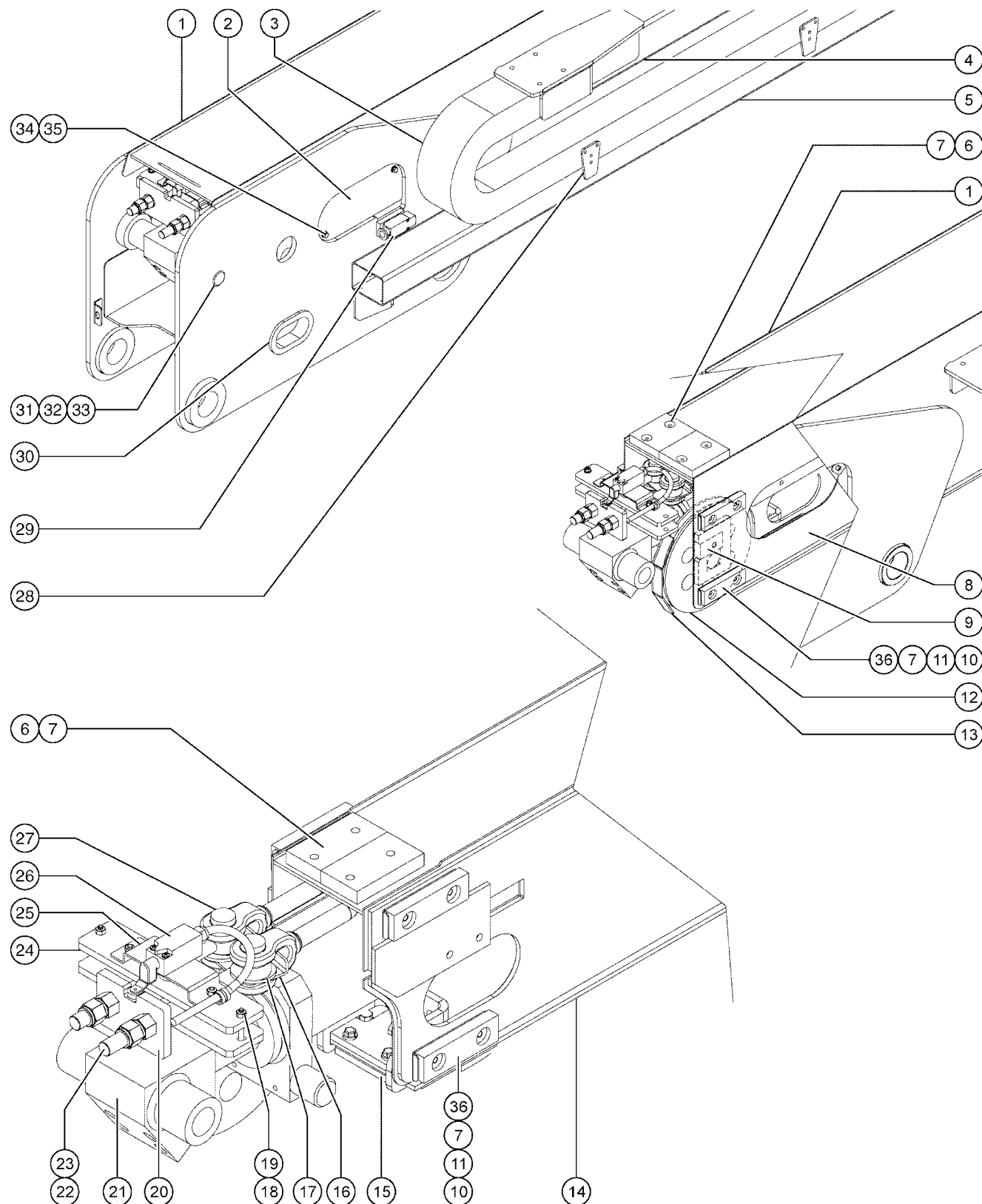
602.1 Boom Components, View 1
